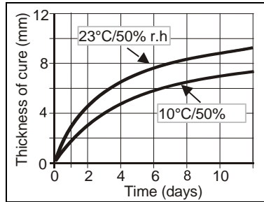
Diagram 1: Curing speed for Sikaflex®-298
